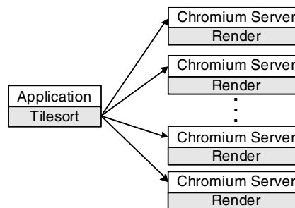
Figure 1: A simple Chromium configuration. In this example, a serial application is made to run on a tiled display using a sort-first stream processor called tilestort .
